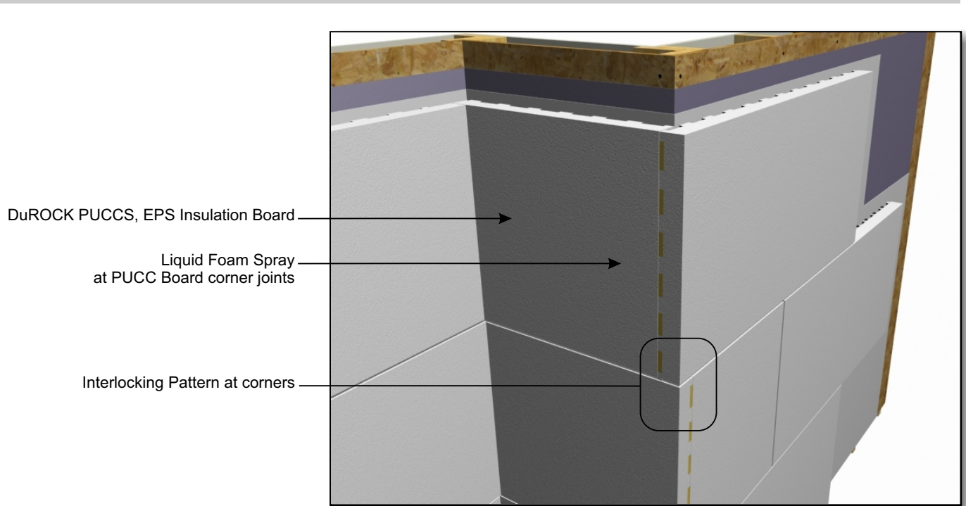
PUCCS-LRRC (17) CORNER TREATMENT, PUCS BOARD INTERLOCKING PATTERN
