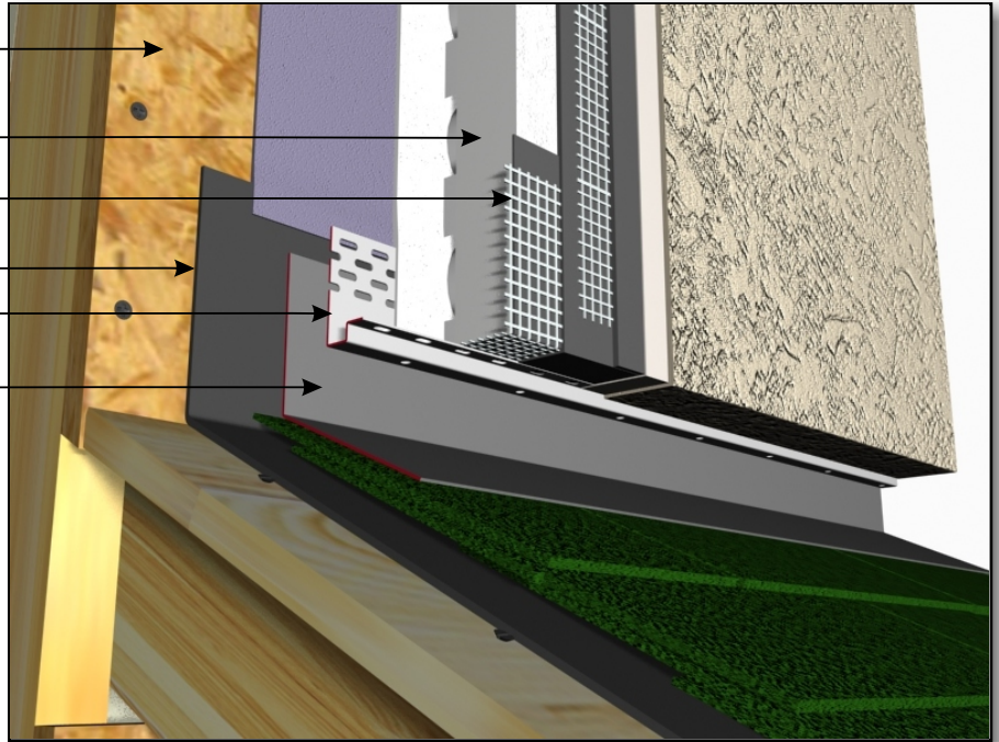
PUCCS-LRRC (10) TERMINATION AT SLOPED ROOF TO FRONT WALL
