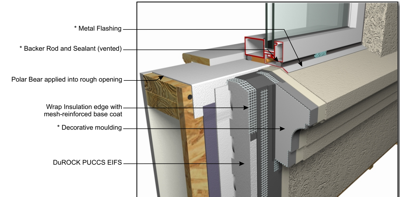
PUCCS-LRRC (04) WINDOW SILL WITH METAL FLASHING
