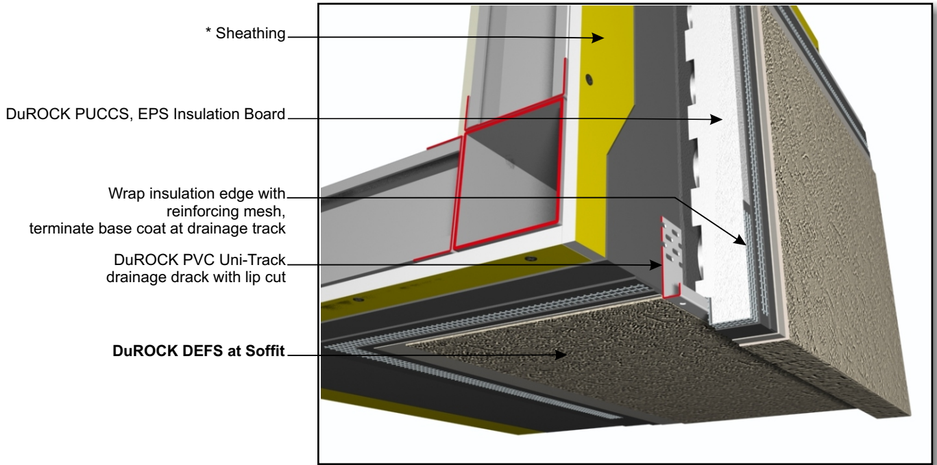
CHRC D10, EIFS TERMINATION AT SOFFIT
