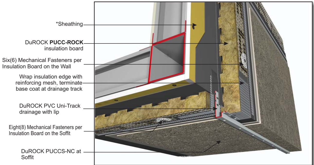
D12, TERMINATION AT SOFFIT
