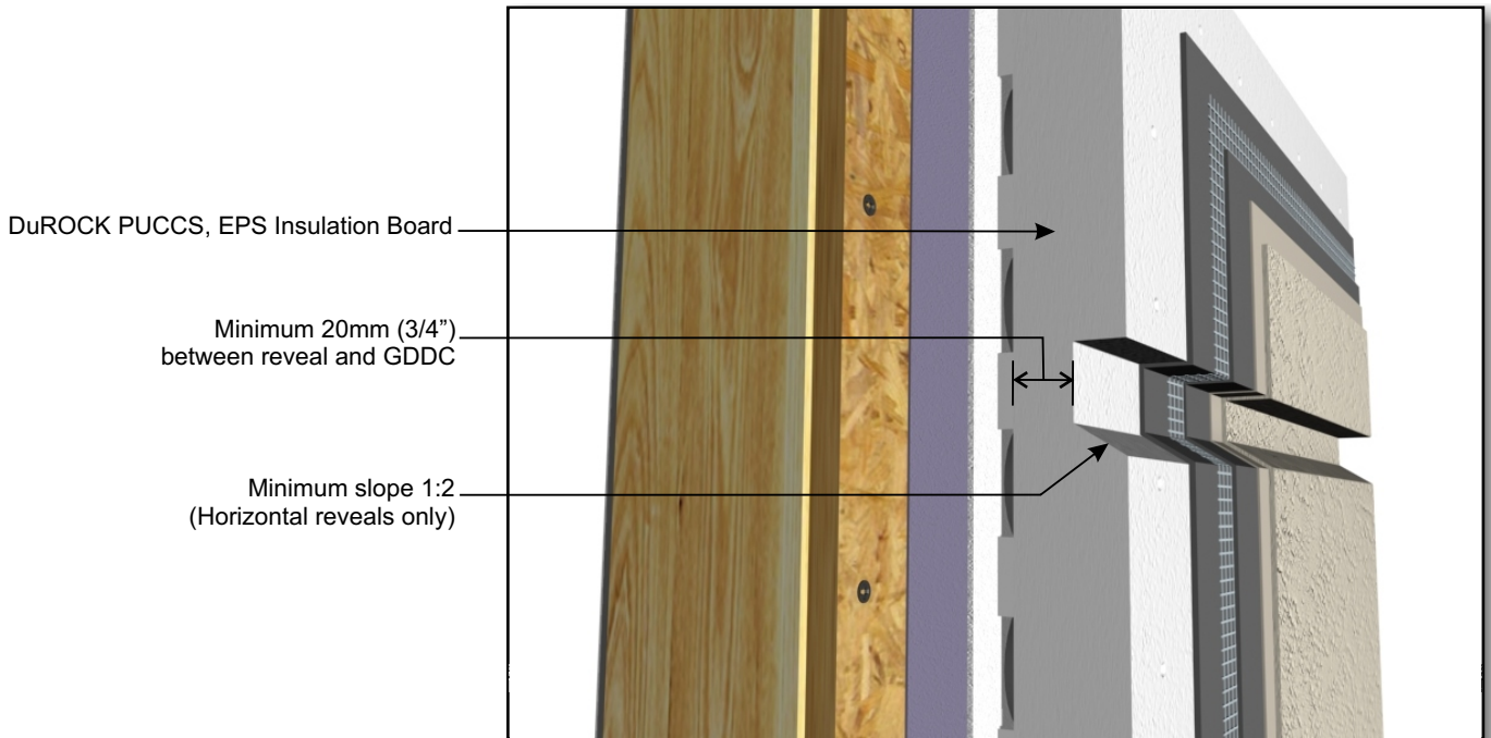
PUCCS-LRRC (13) AESTHETIC REVEAL (TYPE B)
