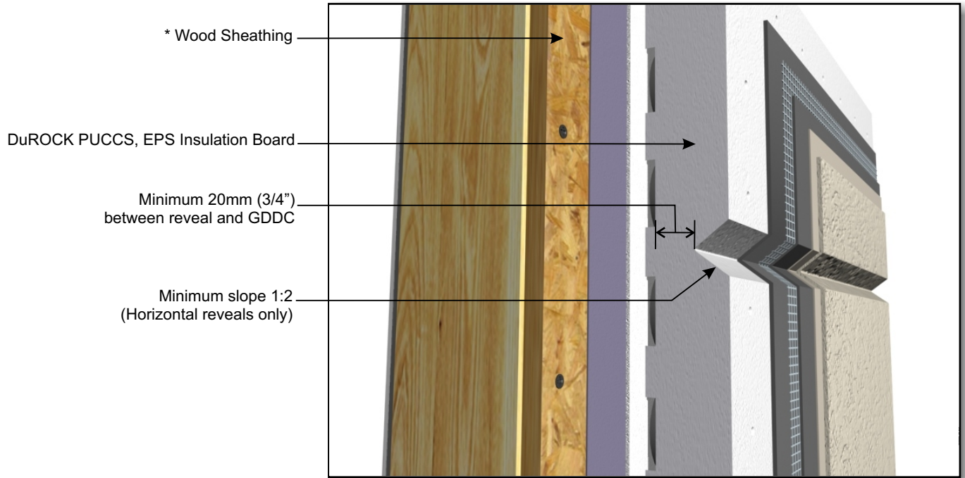
PUCCS-LRRC (13) AESTHETIC REVEAL (TYPE A)
