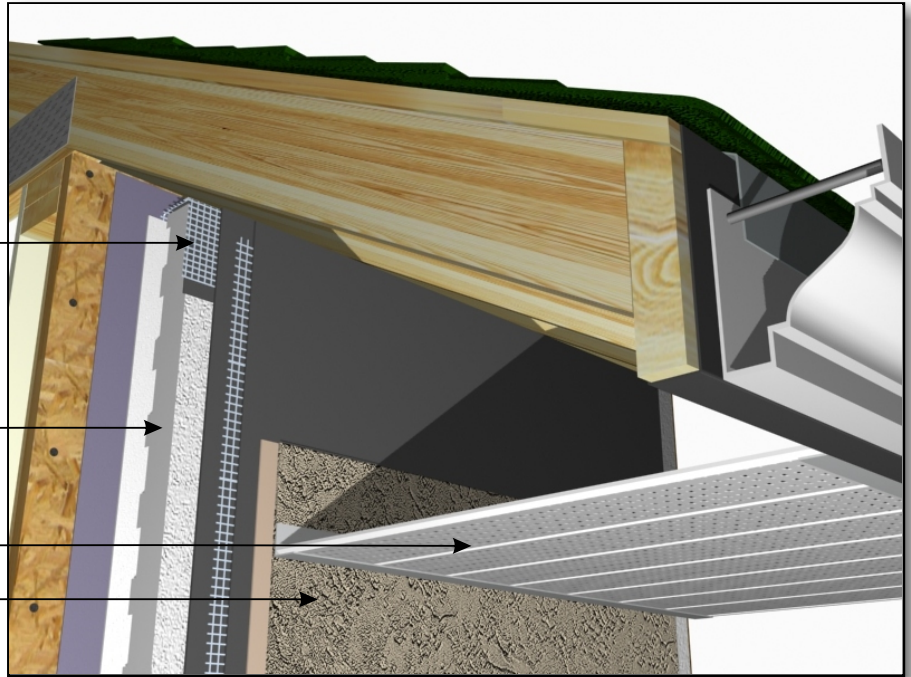
PUCCS-LRRC (10) TERMINATION AT SOFFIT
