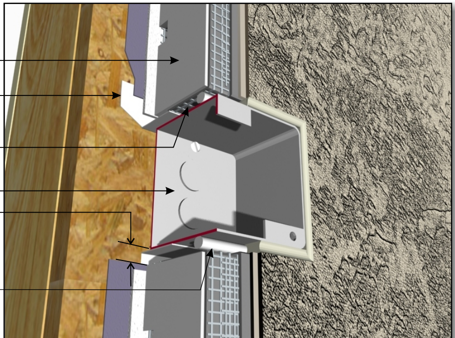
PUCCS-LRRC (11) EXTERIOR ELECTRIC BOX PENETRATION
