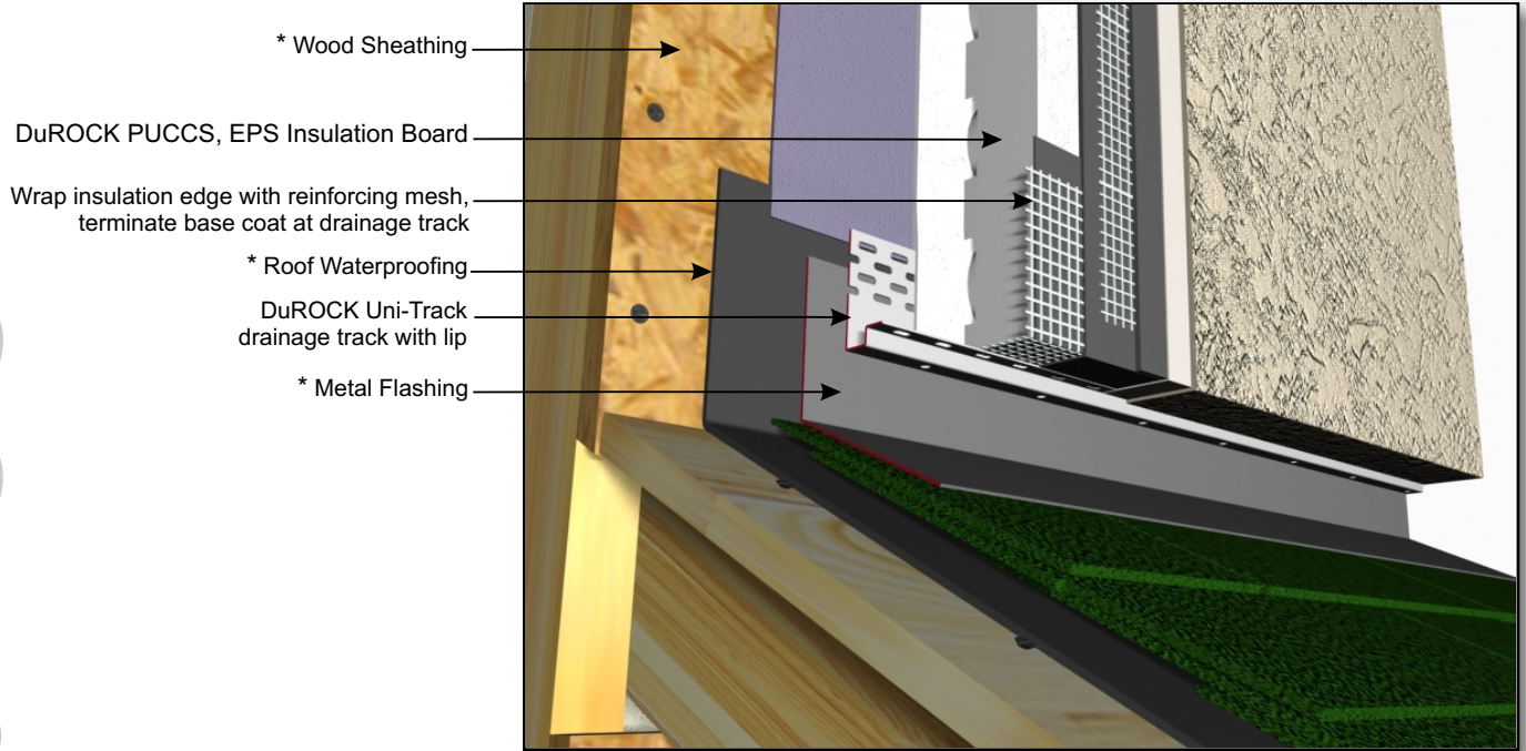
PUCCS-LRRC (07A) TERMINATION AT SLOPED ROOF TO FRONT WALL
