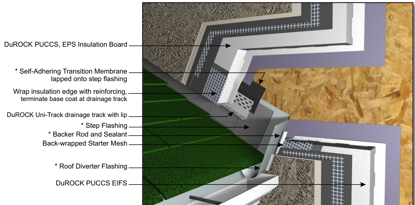
PUCCS-LRRC (07B) TERMINATION AT SLOPED ROOF TO SIDE WALL
