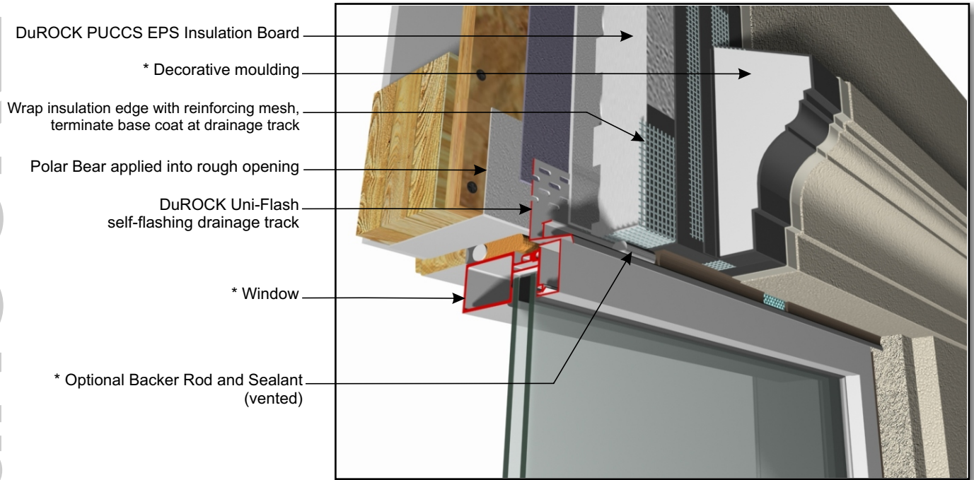
PUCCS LRRC (01A) WINDOW HEADER WITH DuROCK PVC UNI-FLASH
