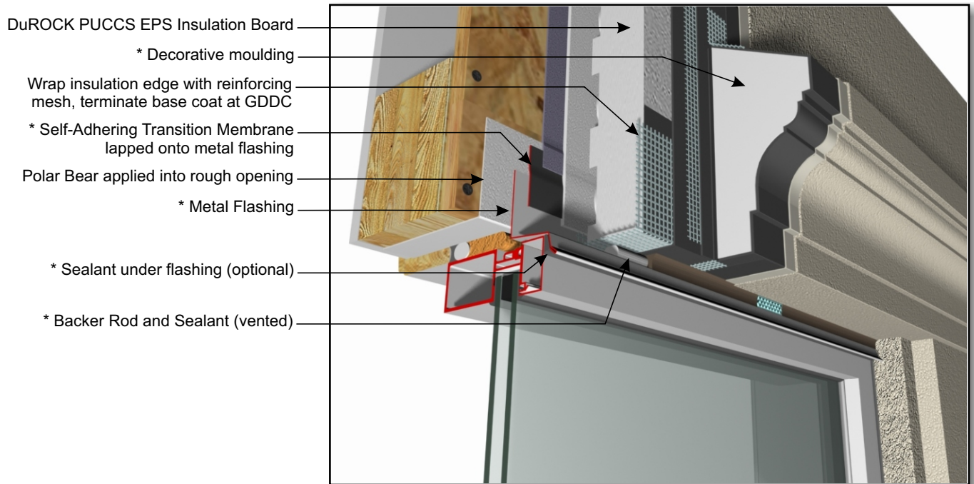
PUCCS-LRRC (01B) WINDOW HEADER WITH METAL FLASHING
