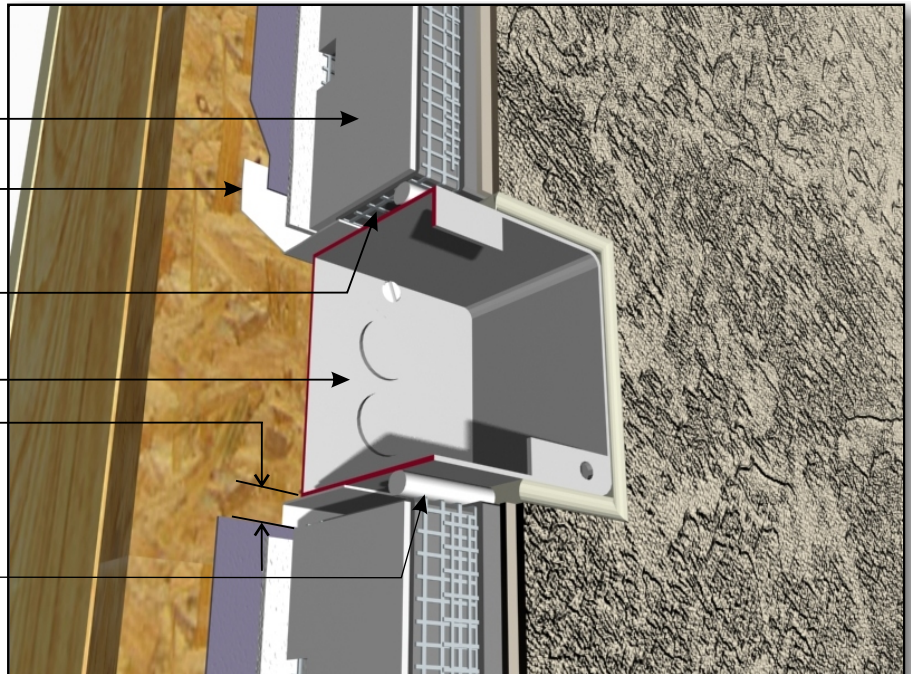
PUCCS-LRRC (16) EXTERIOR ELECTRIC BOX PENETRATION
