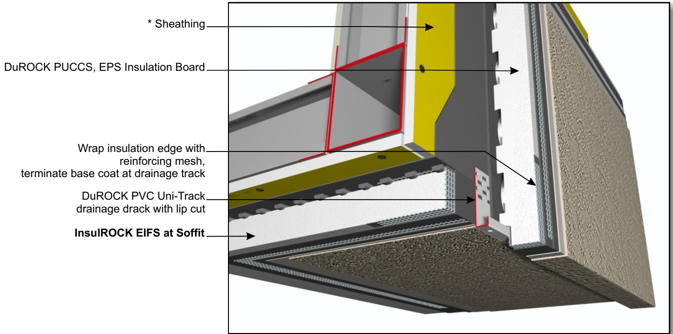
CHRC D10, TERMINATION AT EIFS SOFFIT
