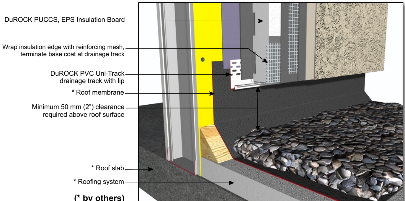
CHRC D08, EIFS TERMINATION AT FLAT ROOF
