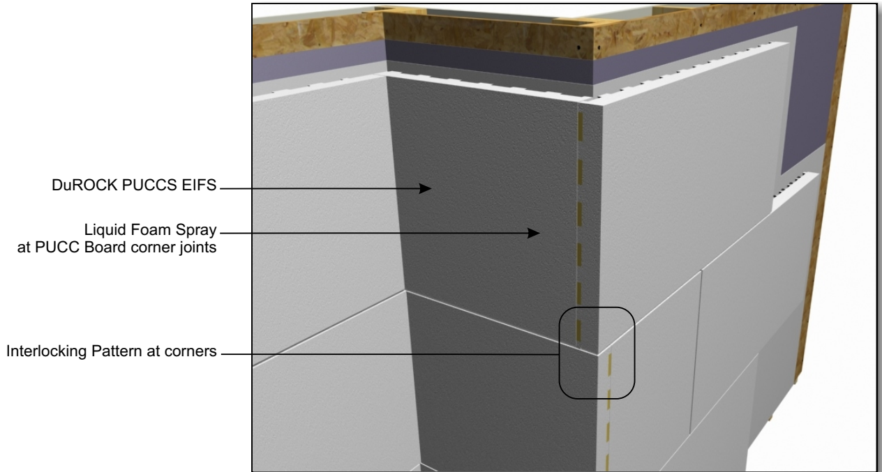
PUCCS-LRRC (16) CORNER TREATMENT, PUCS BOARD INTERLOCKING PATTERN
