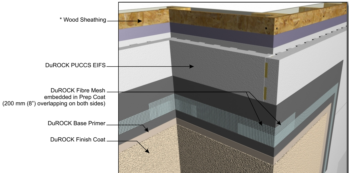
PUCCS-LRRC (16A) CORNER TREATMENT, FIBRE MESH APPLICATION
