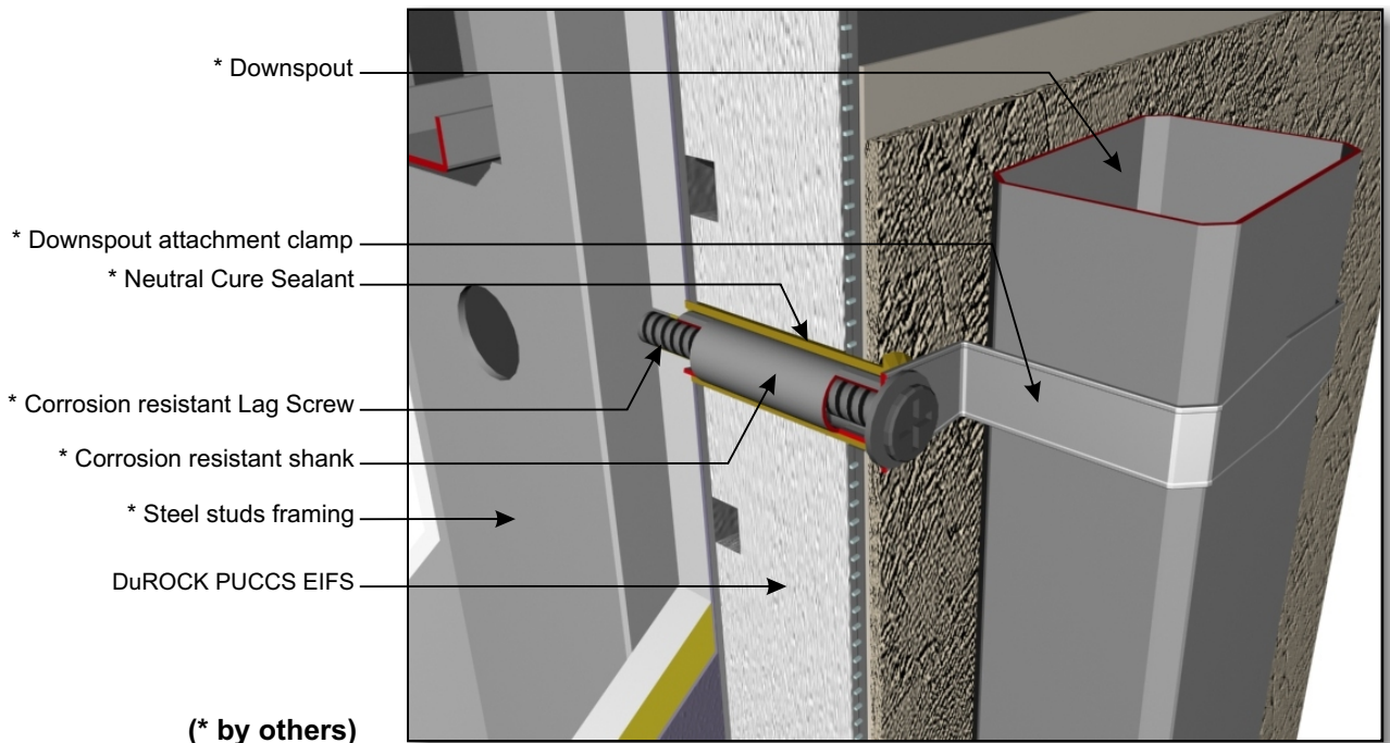
CHRC D14-A, DOWN SPOUT ATTACHMENT
