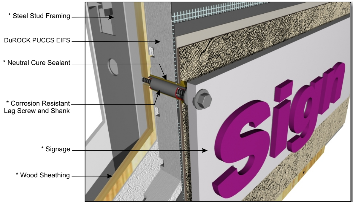
CHRC D14, SIGNAGE ATTACHMENT
