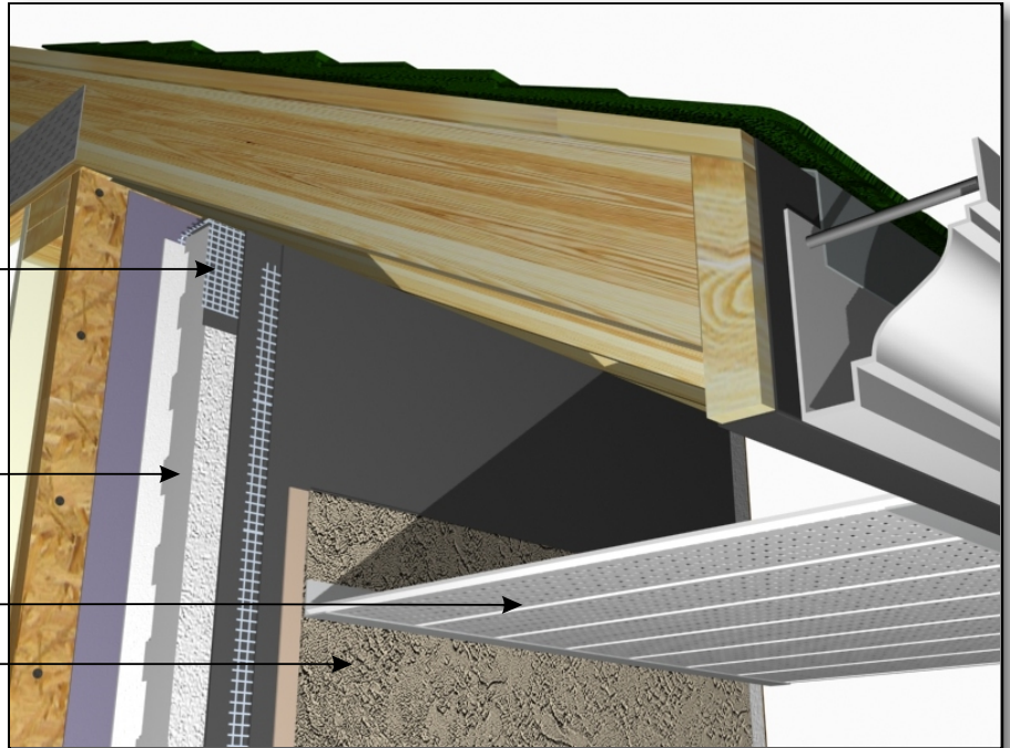
PUCCS-LRRC (14) TERMINATION AT SOFFIT
