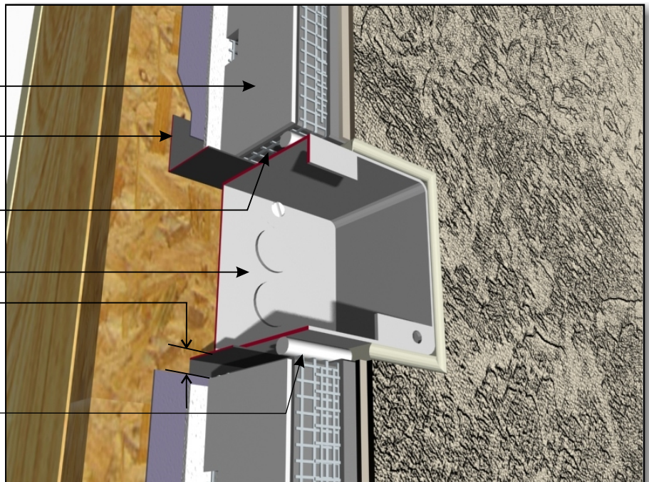
PUCCS-LRRC (15) EXTERIOR ELECTRIC BOX PENETRATION
