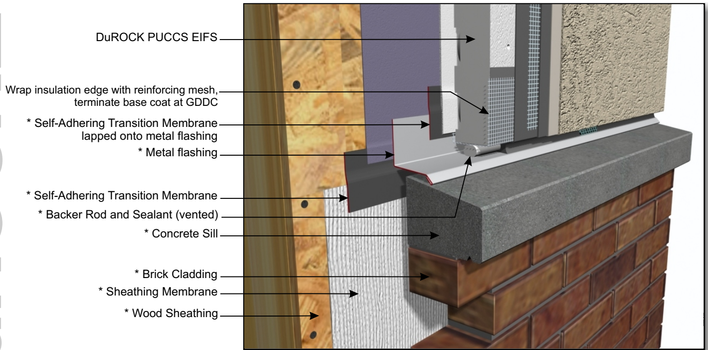
PUCCS-LRRC (12) TERMINATION AT CONCRETE SILL WITH METAL FLASHING
