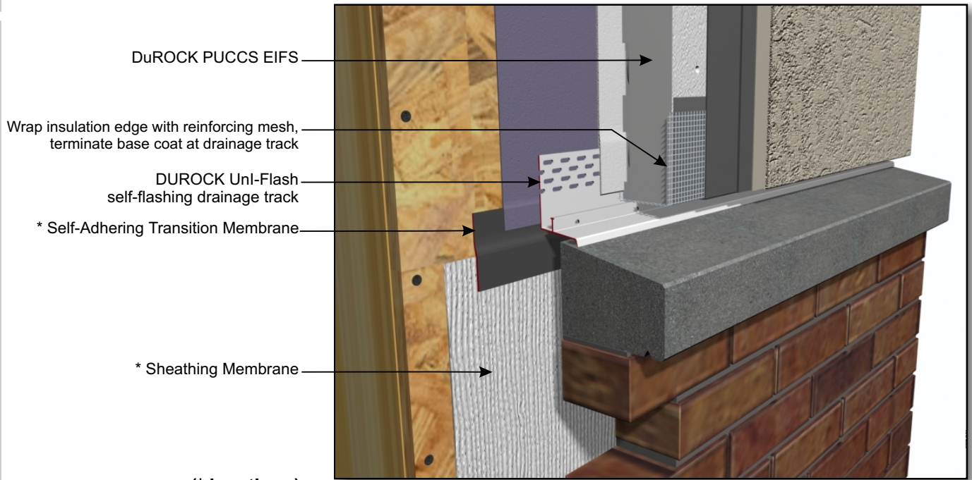
PUCCS-LRRC (13) TERMINATION AT CONCRETE SILL WITH DuROCK UNI-FLASH
