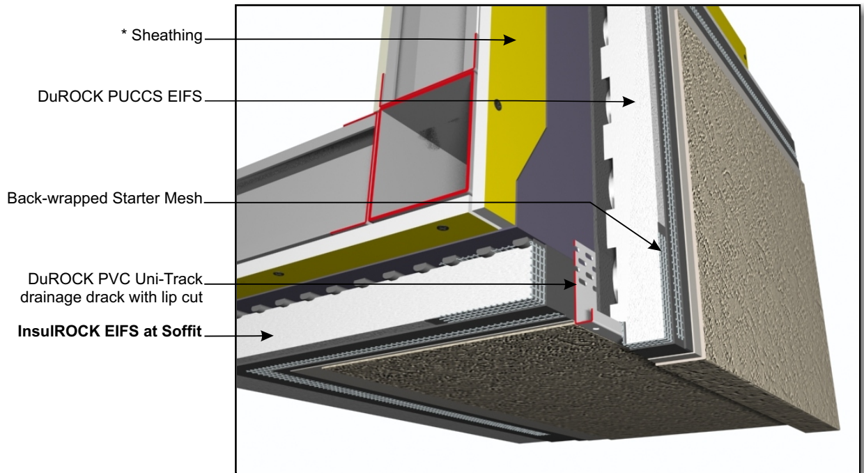
CHRC D10, TERMINATION AT EIFS SOFFIT
