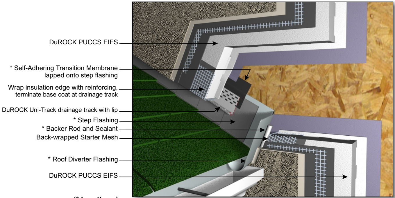
PUCCS-LRRC (11A) TERMINATION AT SLOPED ROOF TO SIDE WALL
