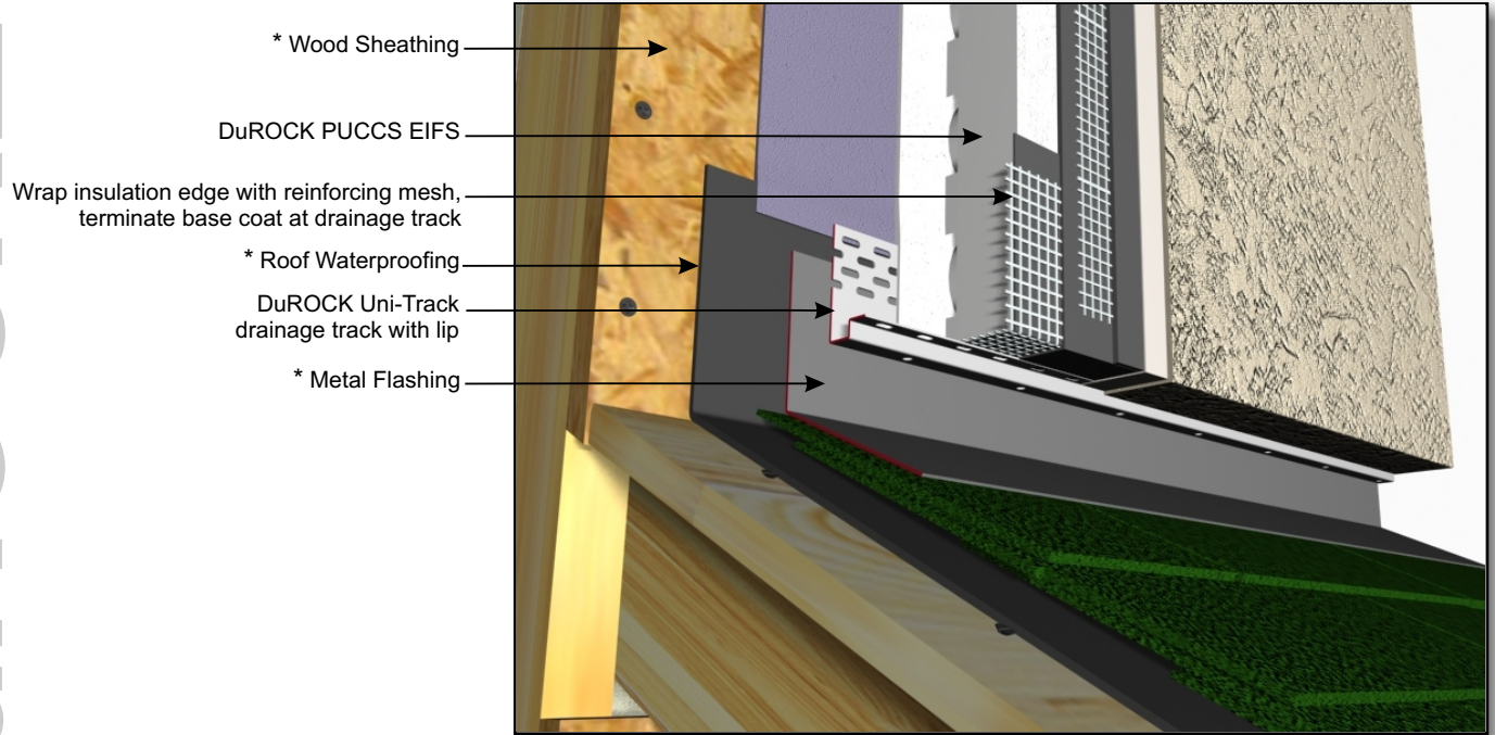
PUCCS-LRRC (11) TERMINATION AT SLOPED ROOF TO FRONT WALL
