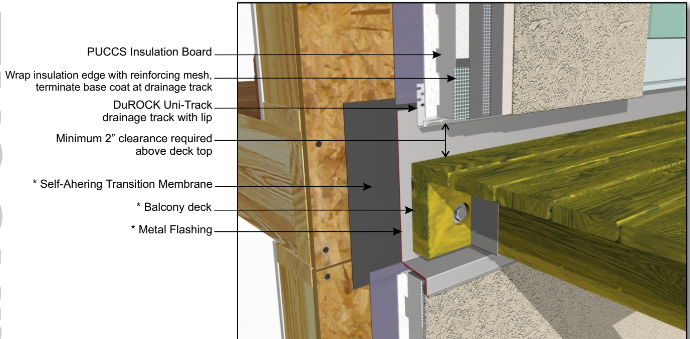
PUCCS-LRRC (09) TERMINATION AT BALCONY/DECK
