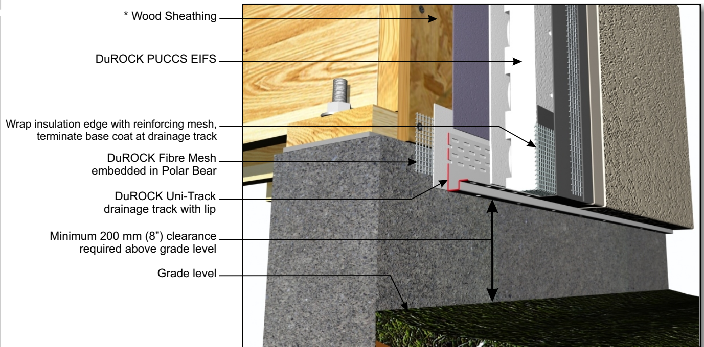
PUCCS-LRRC (10) TERMINATION AT GRADE
