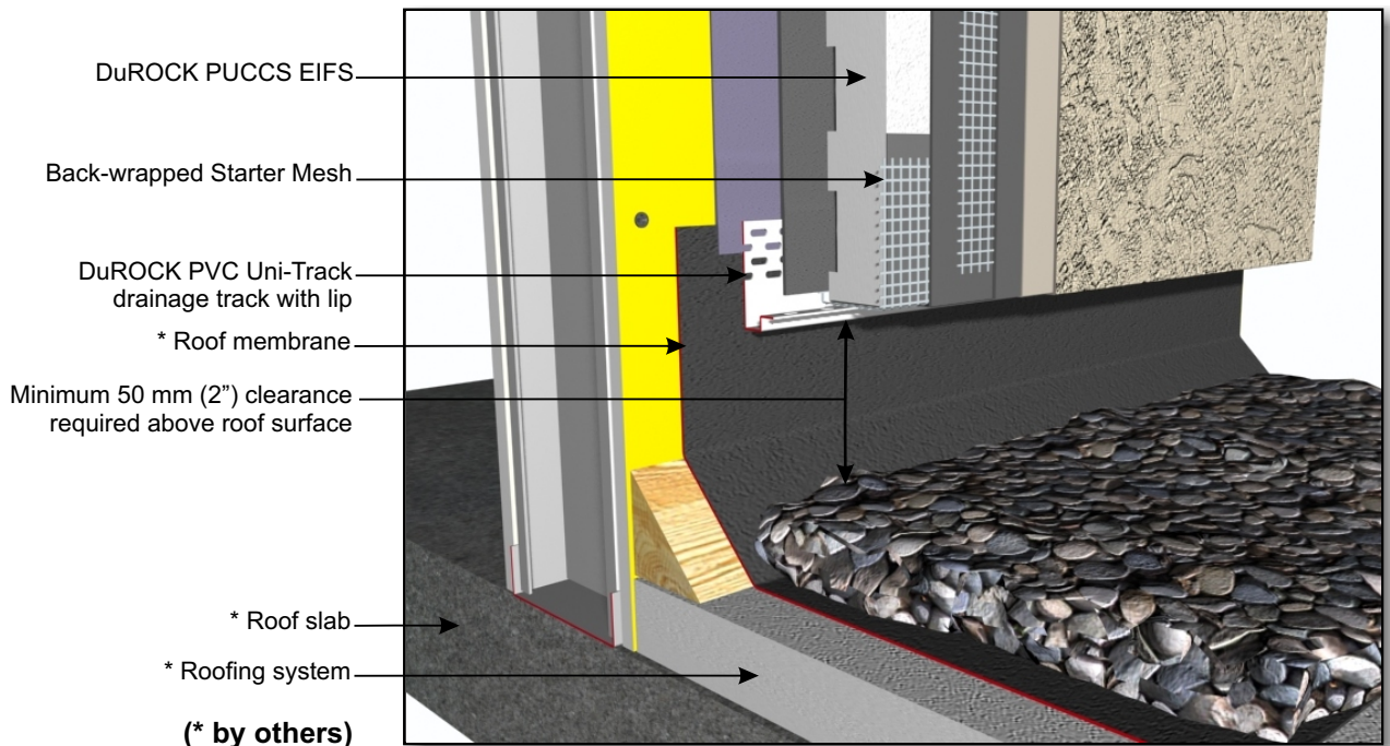
CHRC D08, EIFS TERMINATION AT FLAT ROOF
