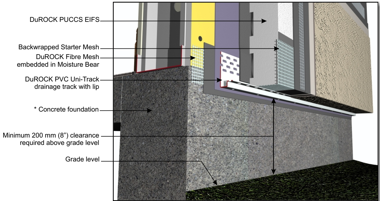
CHRC D07, EIFS TERMINATION AT GRADE
