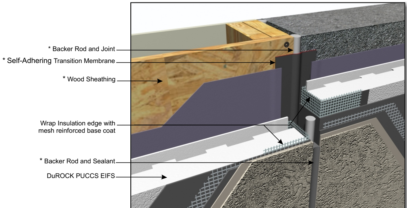
PUCCS-LRRC (08) VERTICAL EXPANSION JOINT, JUNCTION WITH CONCRETE WALL
