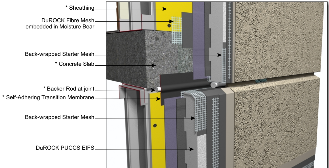
CHREC D05, SEALED HORIZONTAL EXPANSION JOINT
