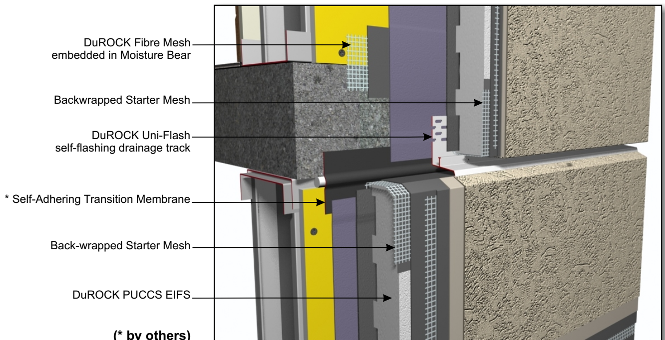
CHRC D06, DRAINED HORIZONTAL EXPANSION JOINT
