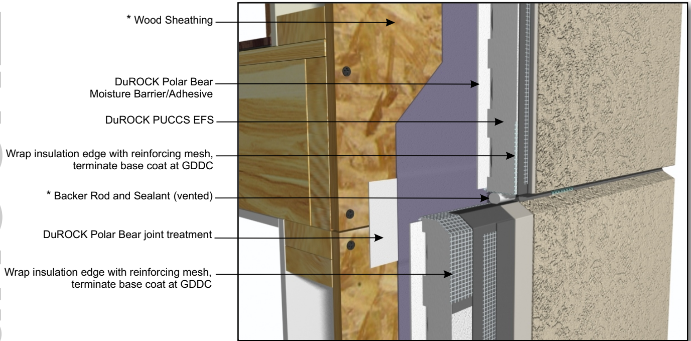
PUCCS-LRRC (05) HORIZONTAL EXPANSION JOINT (SEALED)
