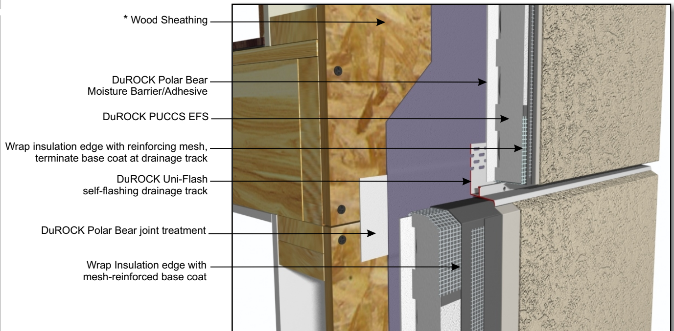
PUCCS-LRRC (06) HORIZONTAL EXPANSION JOINT (DRAINED)
