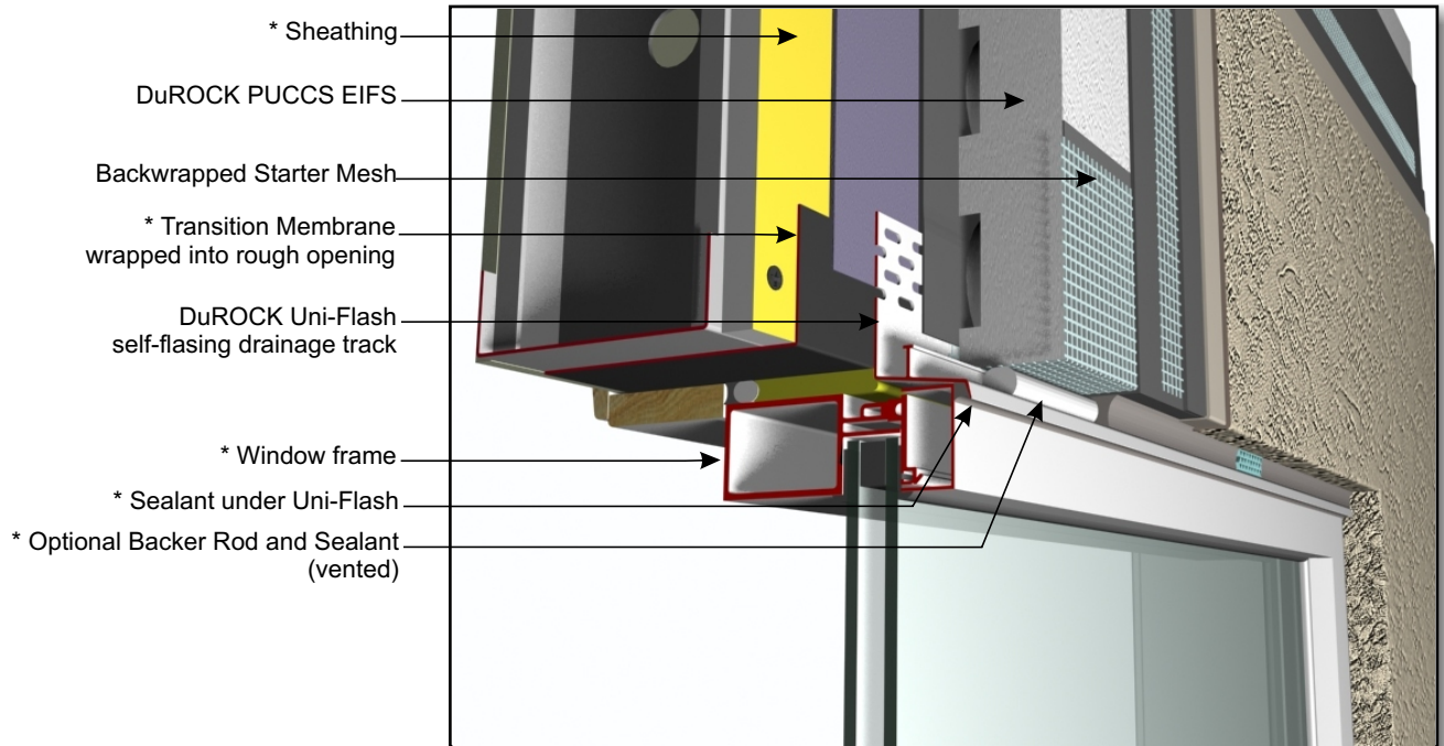
CHRC D01, WINDOW HEADER WITH DuROCK UNI-FLASH
