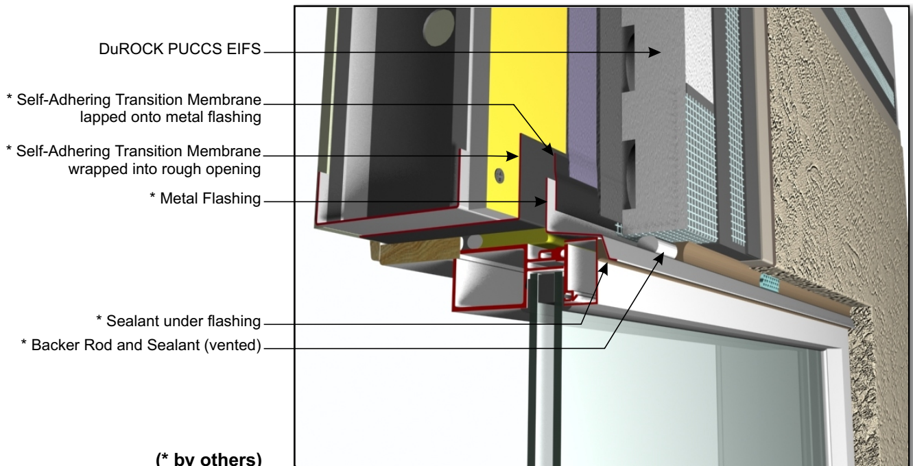
CHRC D02, WINDOW HEADER WITH METAL FLASHING
